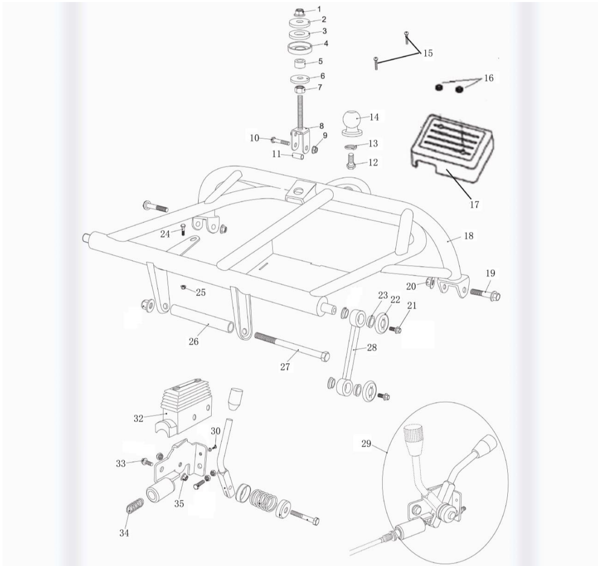
FIG 21: REAR SWING ARM ASSY.UPPER
