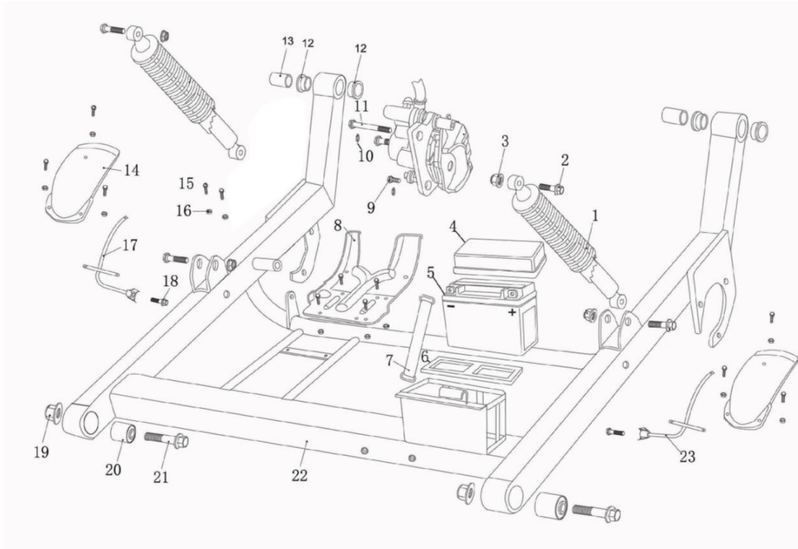
FIG 22: REAR SWING ARM
