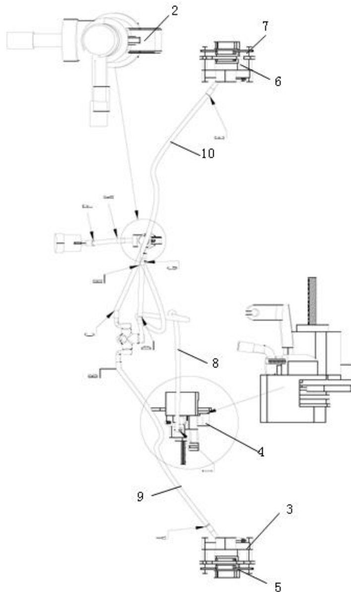
FIG 26 BRAKE ASSY
