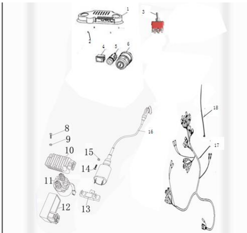
FIG 25 WIRE HARNESS/ELECTRICAL
