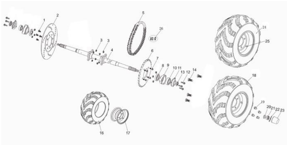
FIG 24 REAR HOUSING
