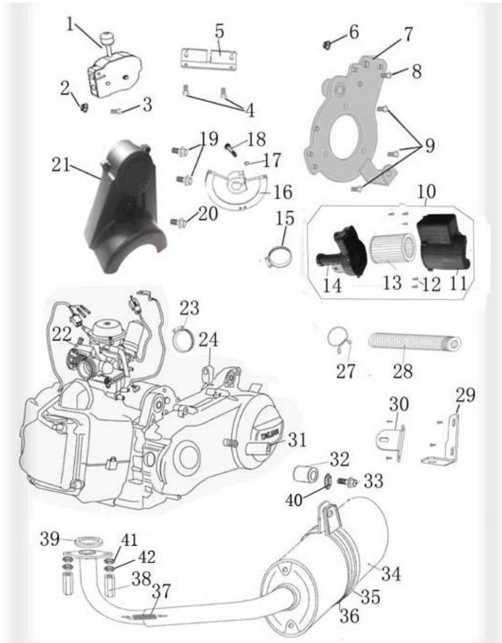
FIG 23: ENGING/MUFFLER/EIR/CLEANER
