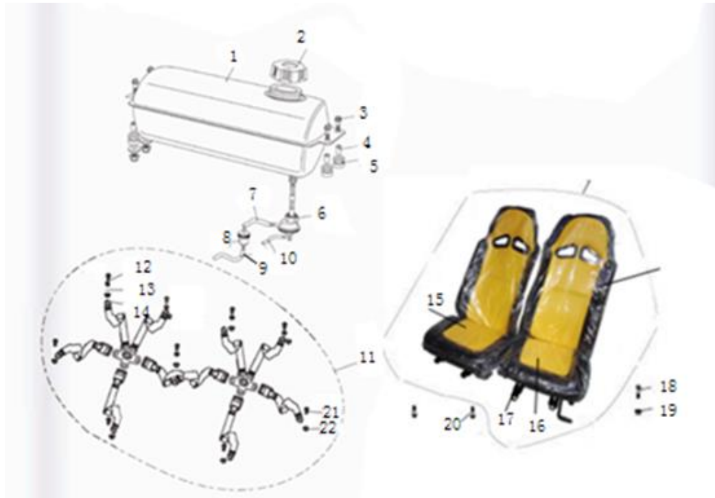
FIG 20: REAR CARGO RACK/SEAT/BELT
