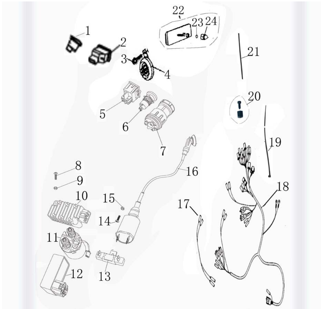
Fig 25 WIRE HARNESS/ELECTRICAL
