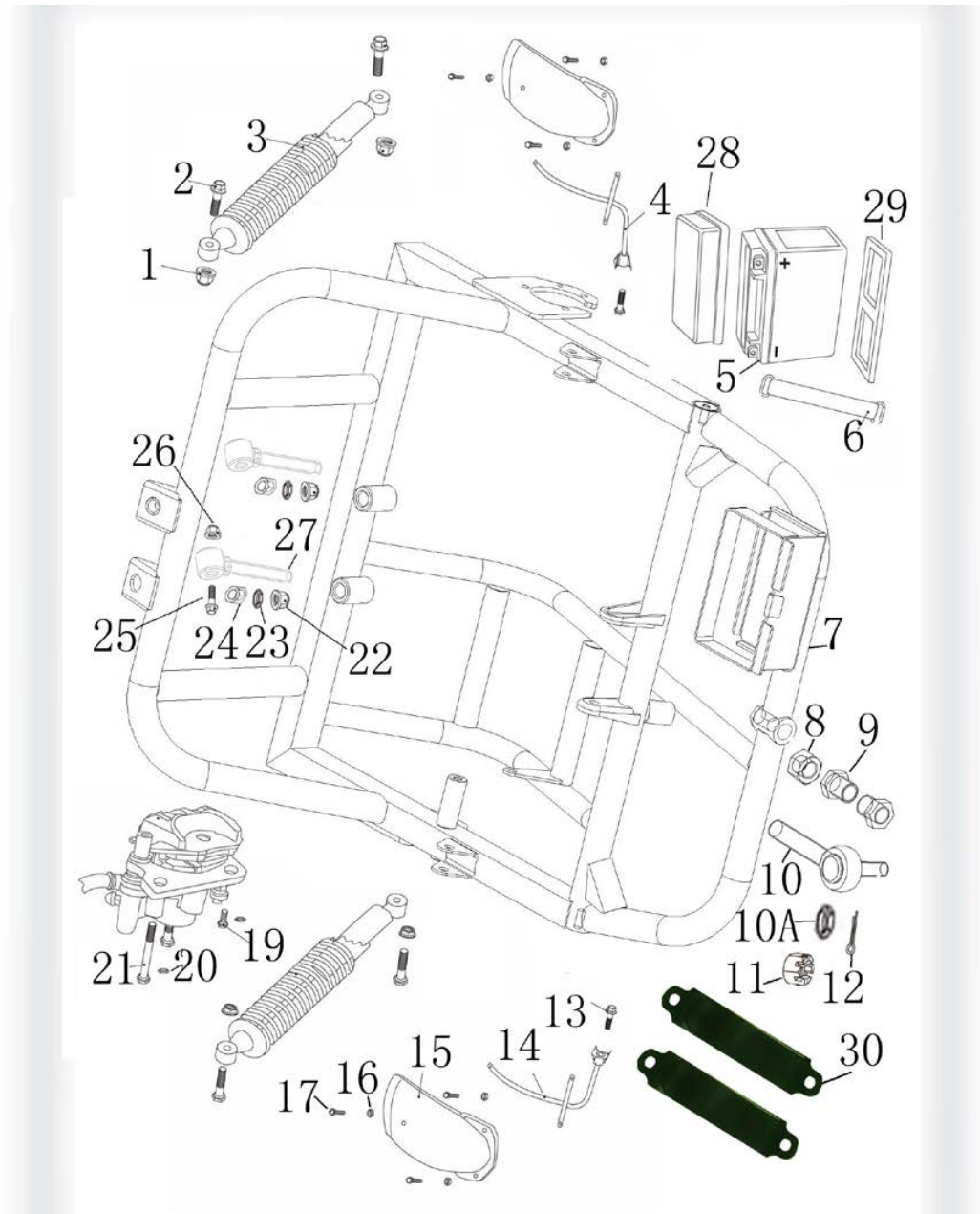
Fig 22: REAR SWING ARM
