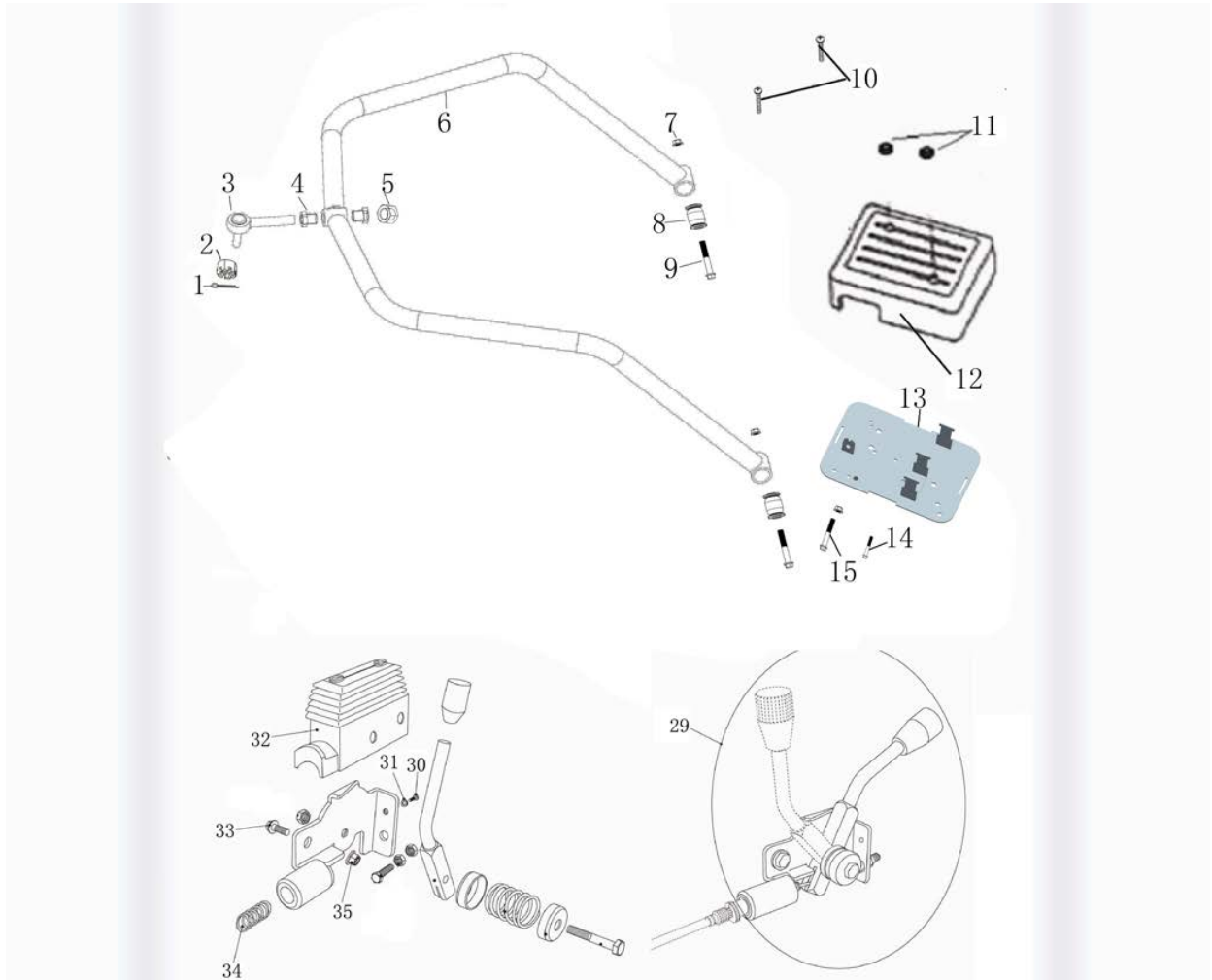
Fig 21: REAR SWING ARM ASSY.UPPER
