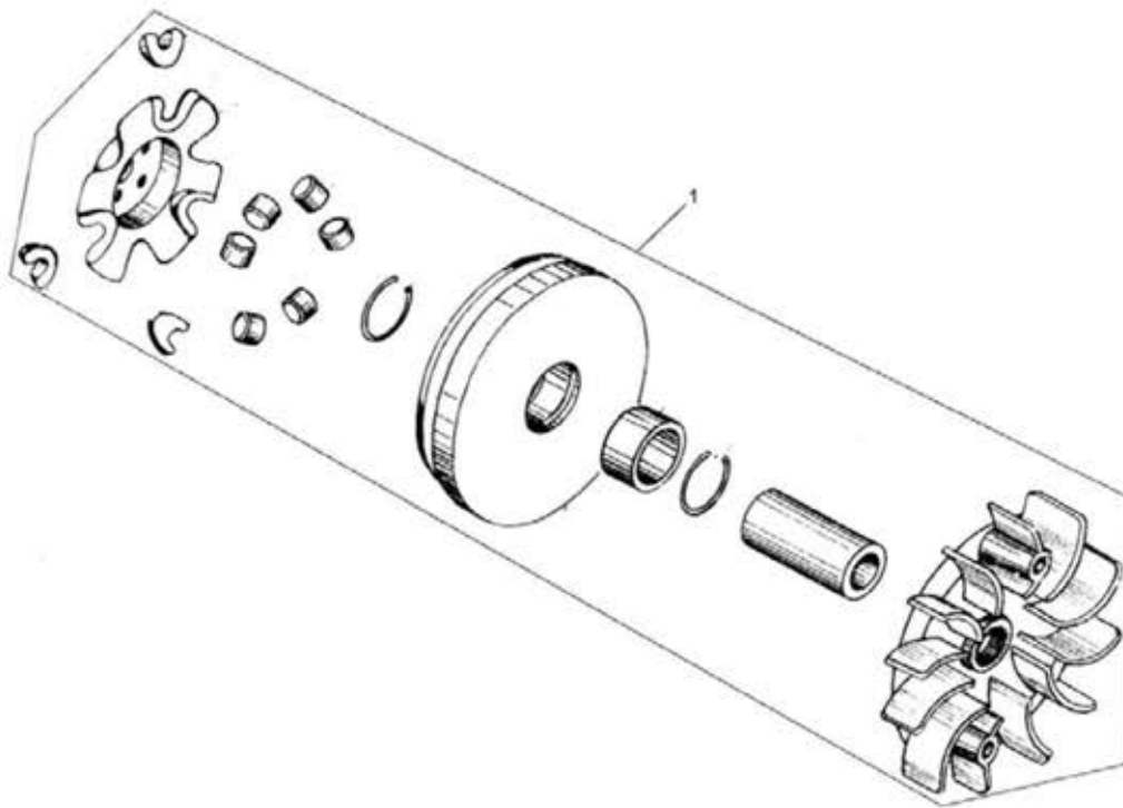
FIG .10 DRIVING WHEEL COMP.
