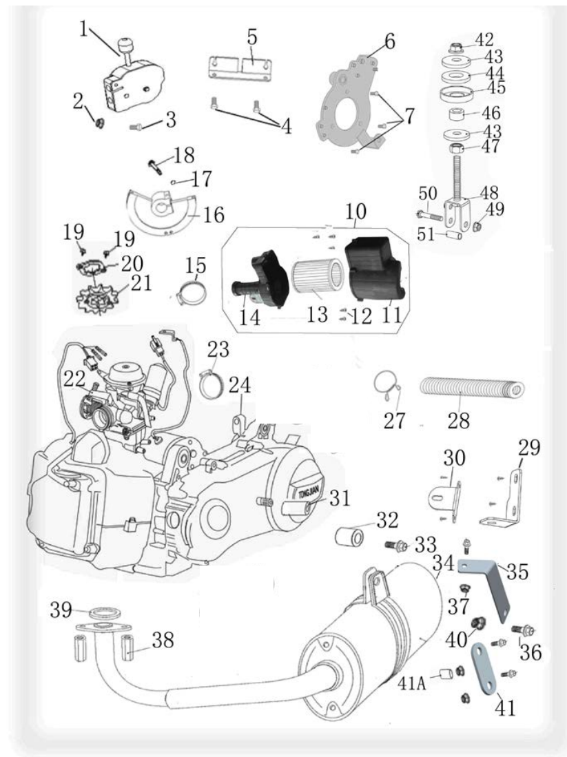
Fig 23: ENGING/MUFFLER/EIR/CLEANE
