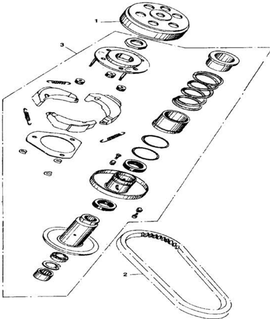
FIG. 12 DRIVEN WHEEL COMP
