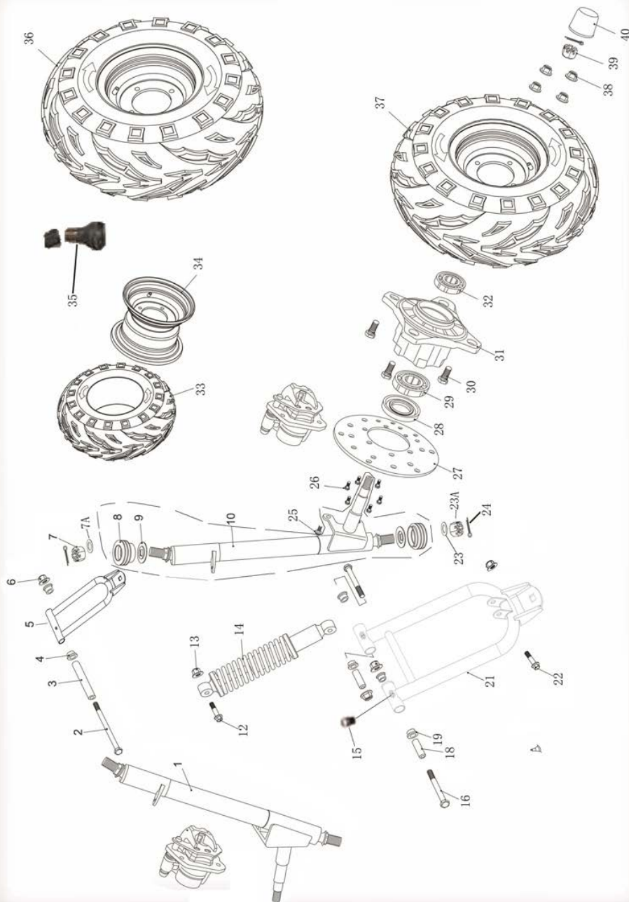
Fig 19: SUSPENSION ARM ASSY
