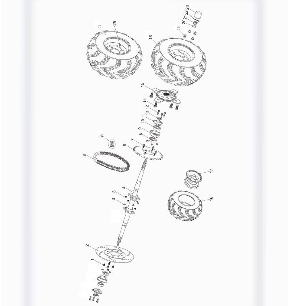
Fig 24 REAR HOUSING
