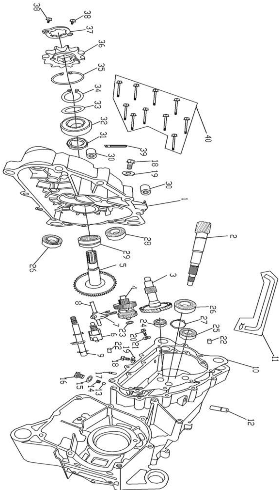
FIG. 2 DRIVING GEAR COMP.
