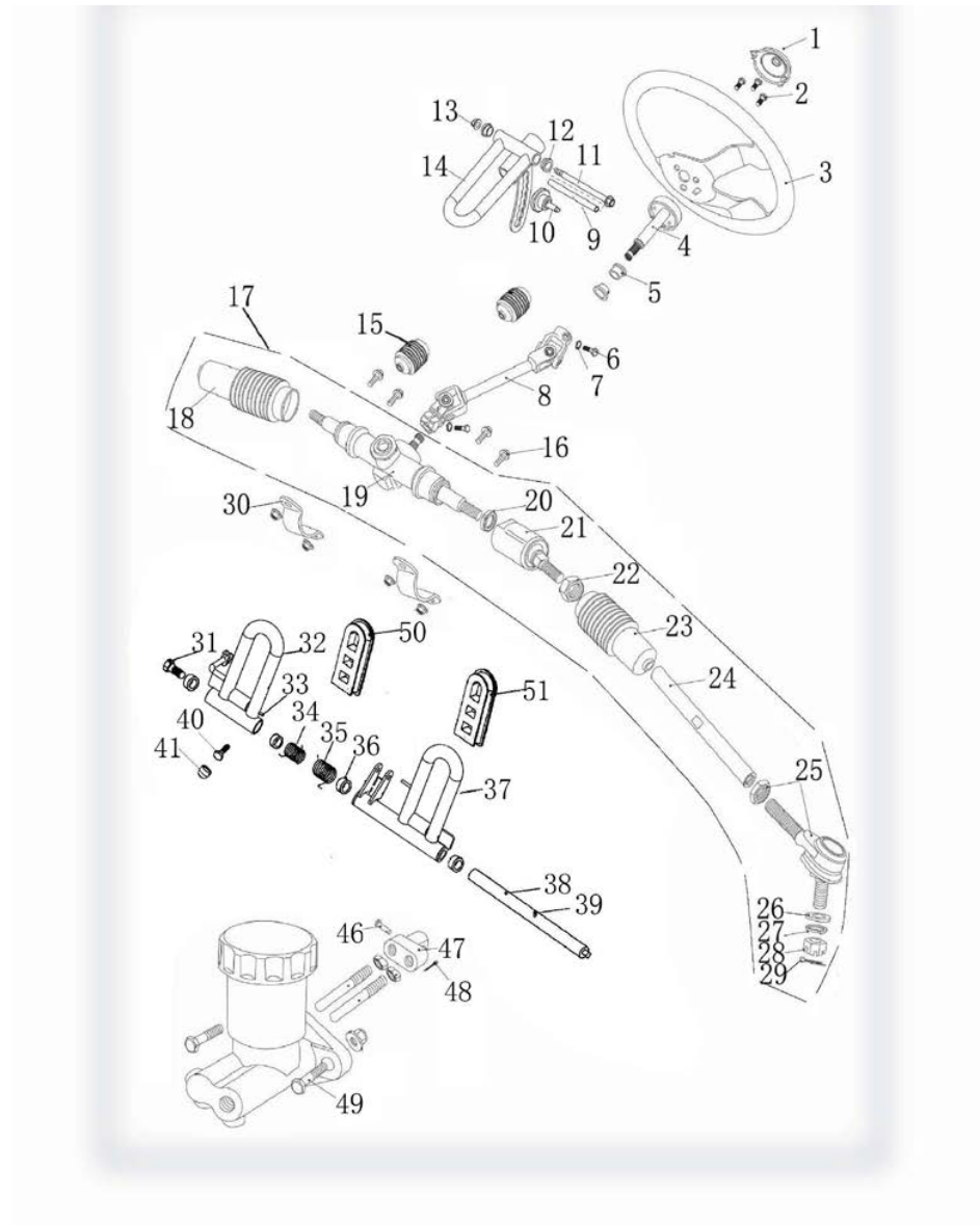
Fig 18: STEERING SHAFT ASSY
