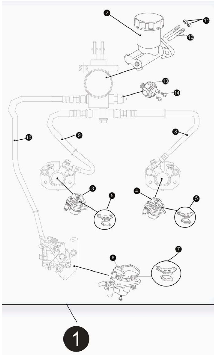
Fig 26 BRAKE ASSY
