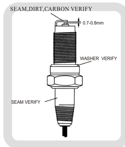
Figure 6 Spark plug
