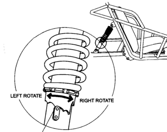
Figure 9 Shock adjustment
